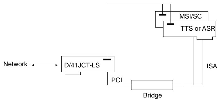
Mixed PCI/ISA Configuration Example
